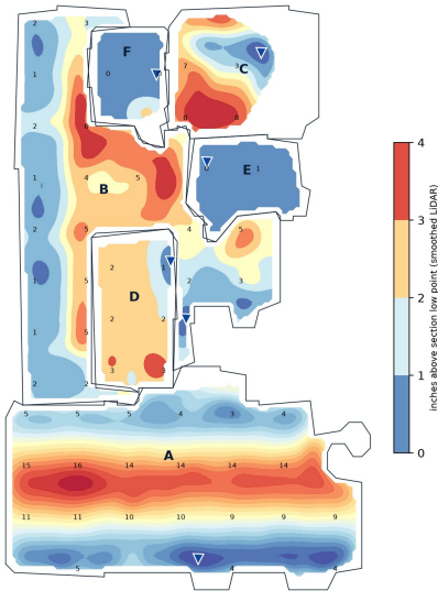
SLOPE-TO-DRAIN MAP (SMOOTHED LiDAR ROOF SURFACE)
